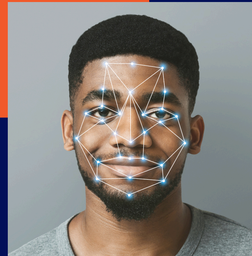
FACE RECOGNITION
